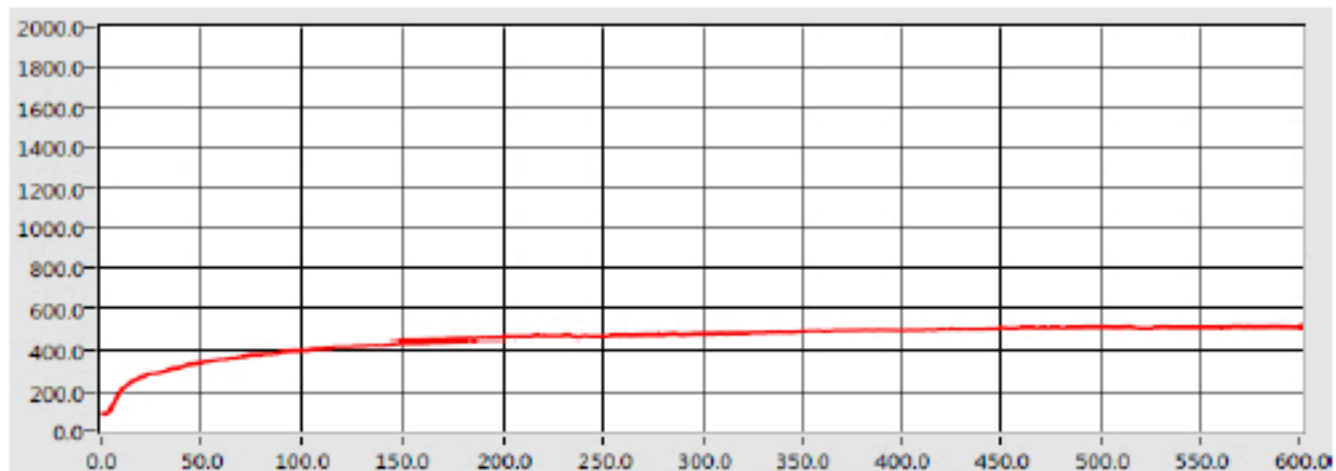
Graph No. 3 - Tunnel Air Temperature Versus Time
